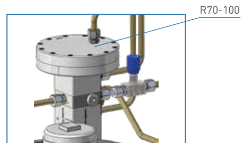
RSP 255 shown with actuator AS 255 incl. control device MD or MD-R and regulator R 70-100
